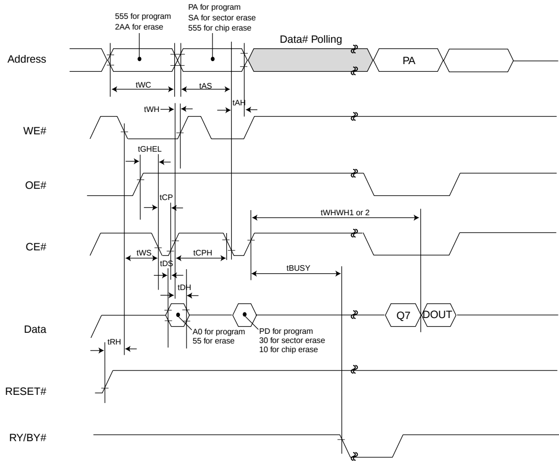
Figure 5. CE# CONTROLLED WRITE TIMING WAVEFORM
