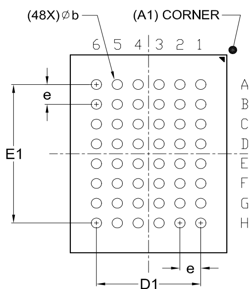
BOTTOM VIEW
