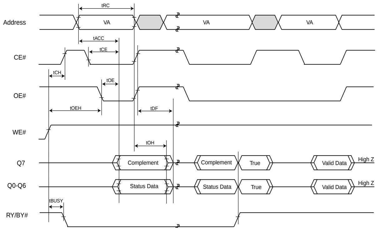
Figure 20. Data# Polling Timings (During Automatic Algorithms)
